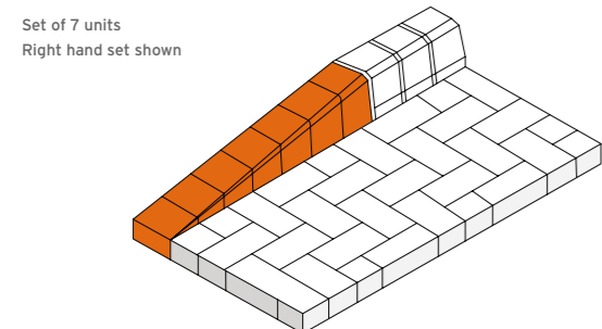
DROP KERB
