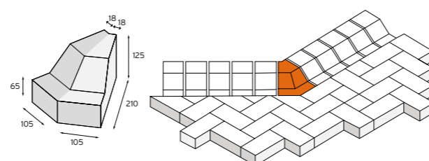
BUCKFAST 45° EXTERNAL RETURN
