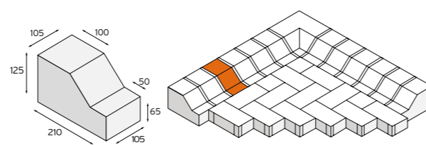
BUCKFAST KERB
