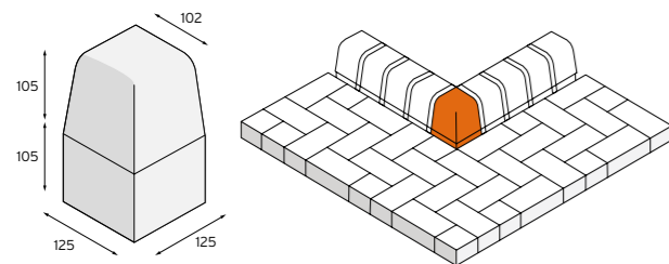
90° INTERNAL RETURN
