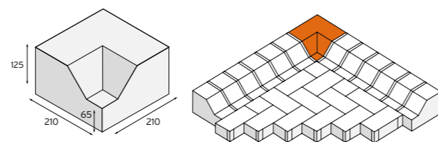
BUCKFAST 45° EXTERNAL RETURN
