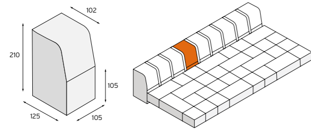
90° EXTERNAL RETURN
