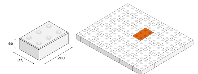
TACTILE PAVER
