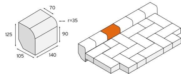
BUCKFAST KERB
