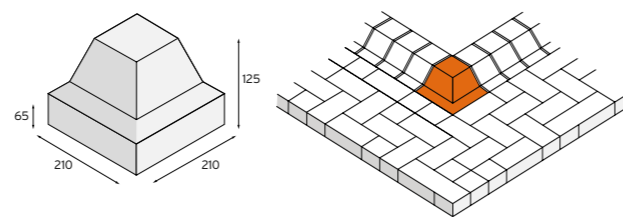
BUCKFAST 90° INTERNAL RETURN
