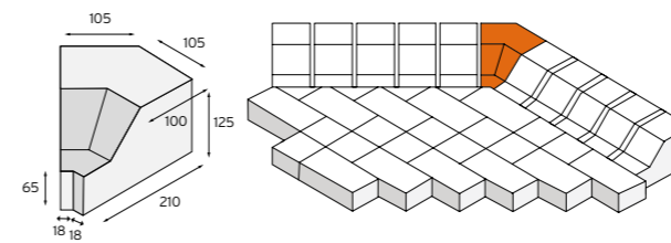
BUCKFAST KERB (LOW) TO STANDARD KERB
