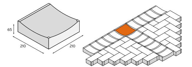
TACTILE PAVER
