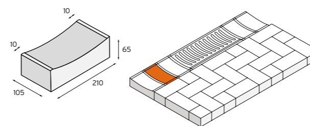
CHANNEL UNIT including Chancast Gulligridd (by other)
